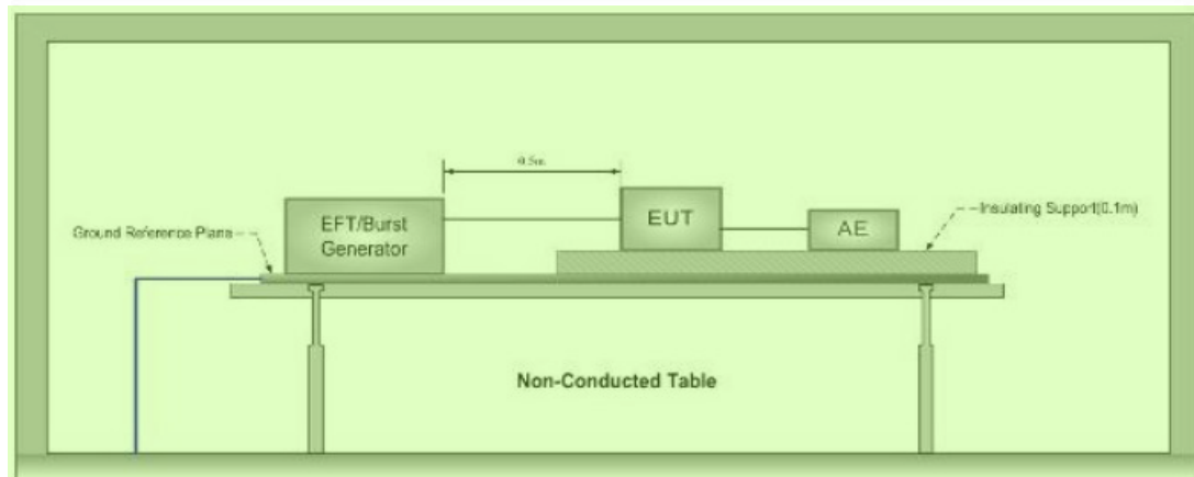
Ground Reference Plane
