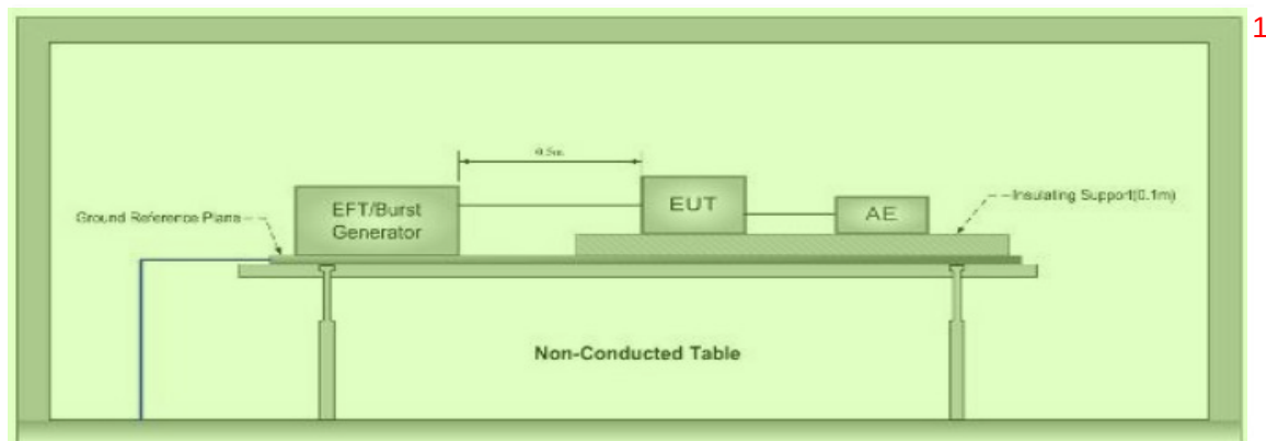
Ground Reference Plane 2
