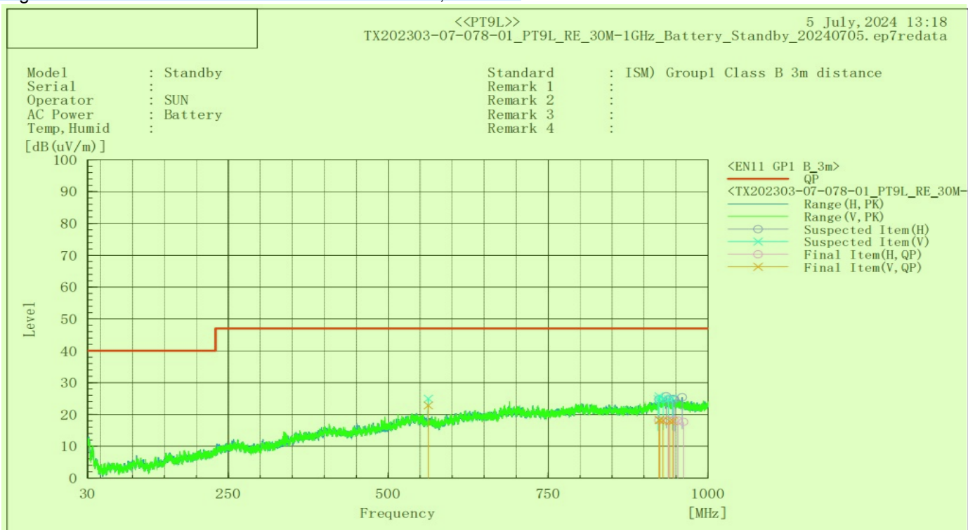
Figure 1: Measurement results of radiated emission, Mode 1 3
