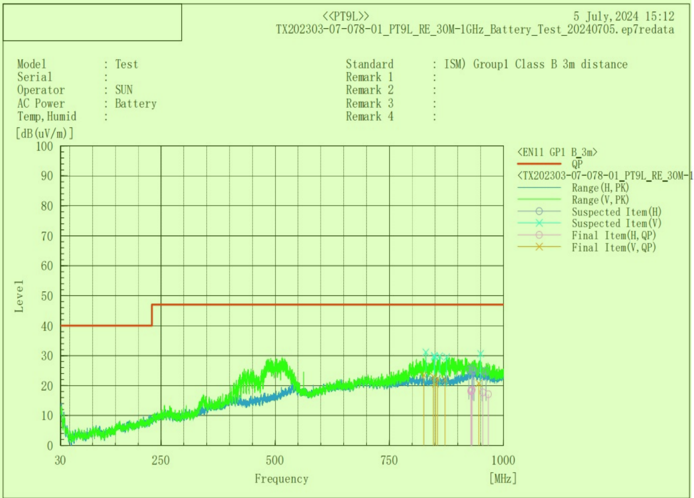
Figure 2: Measurement results of radiated emission, Mode 2
